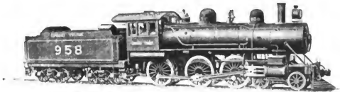
Ten-Wheel Locomotive for Fast Passenger Service Built for Grand Trunk Railway
